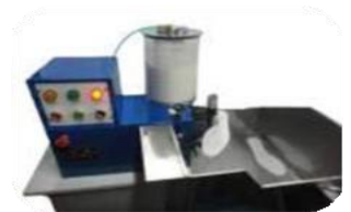
Cement Auto-coating
